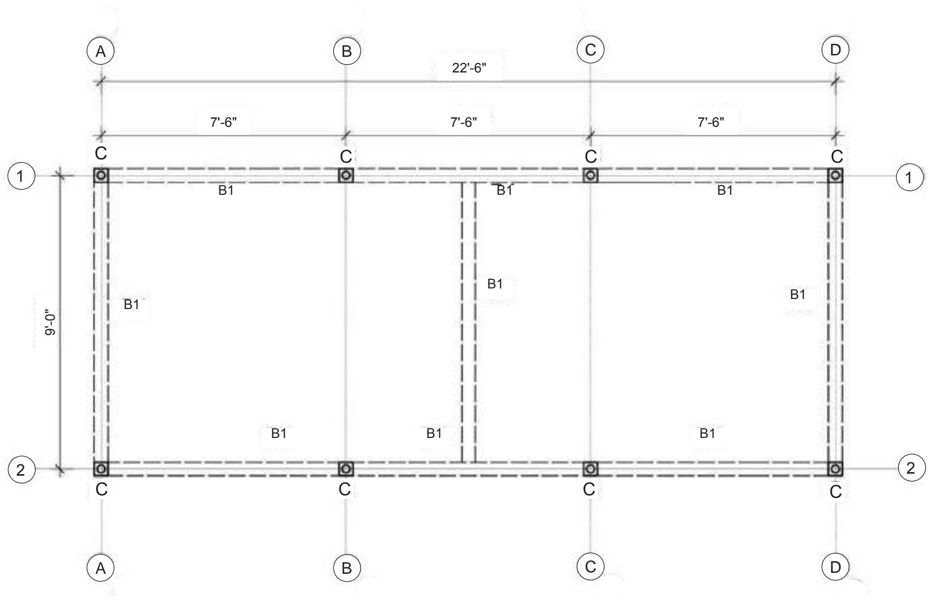
Beam-Column layout
