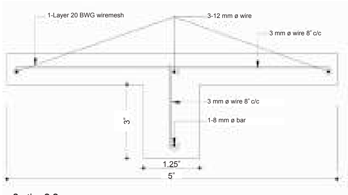
Section C-C
