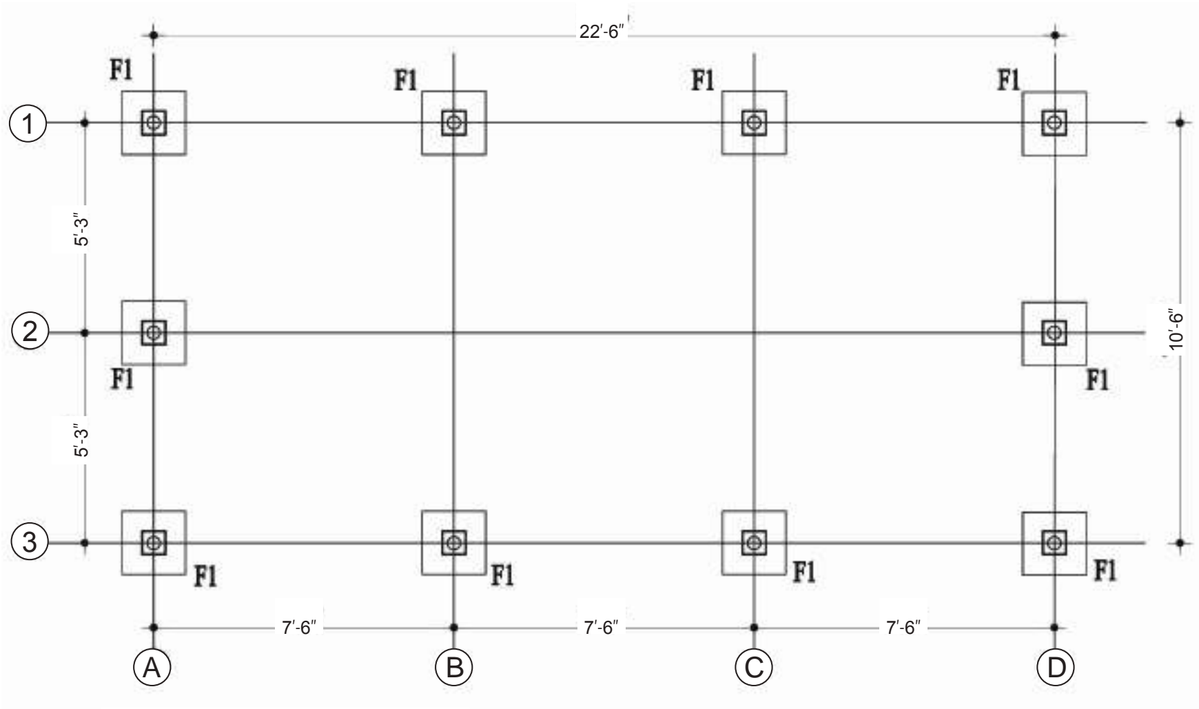
Foundation layout
