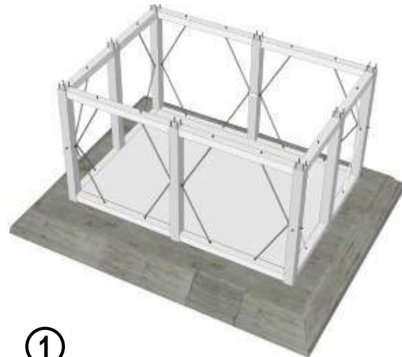
Plinth structural frame
