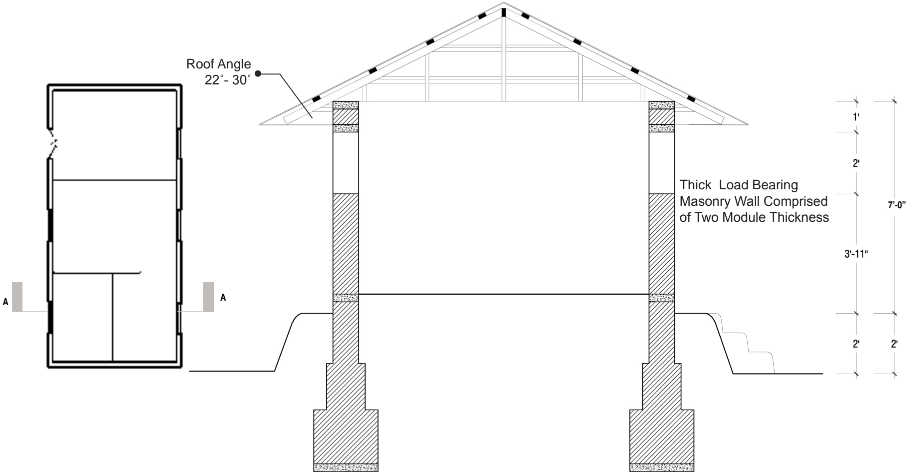
Section AA
