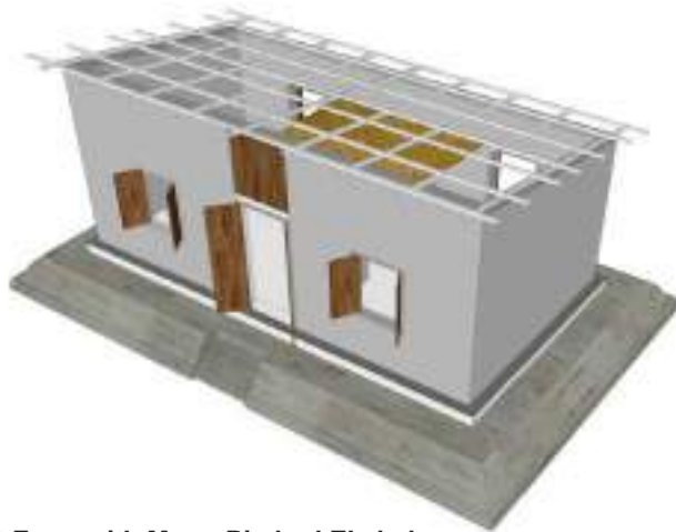
Complete Built Form with Mono Pitched Ekchala Roof for Area 2
